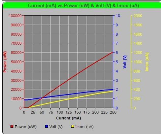
PIV Curve
